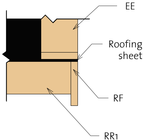
③ Roof Reinforcement
